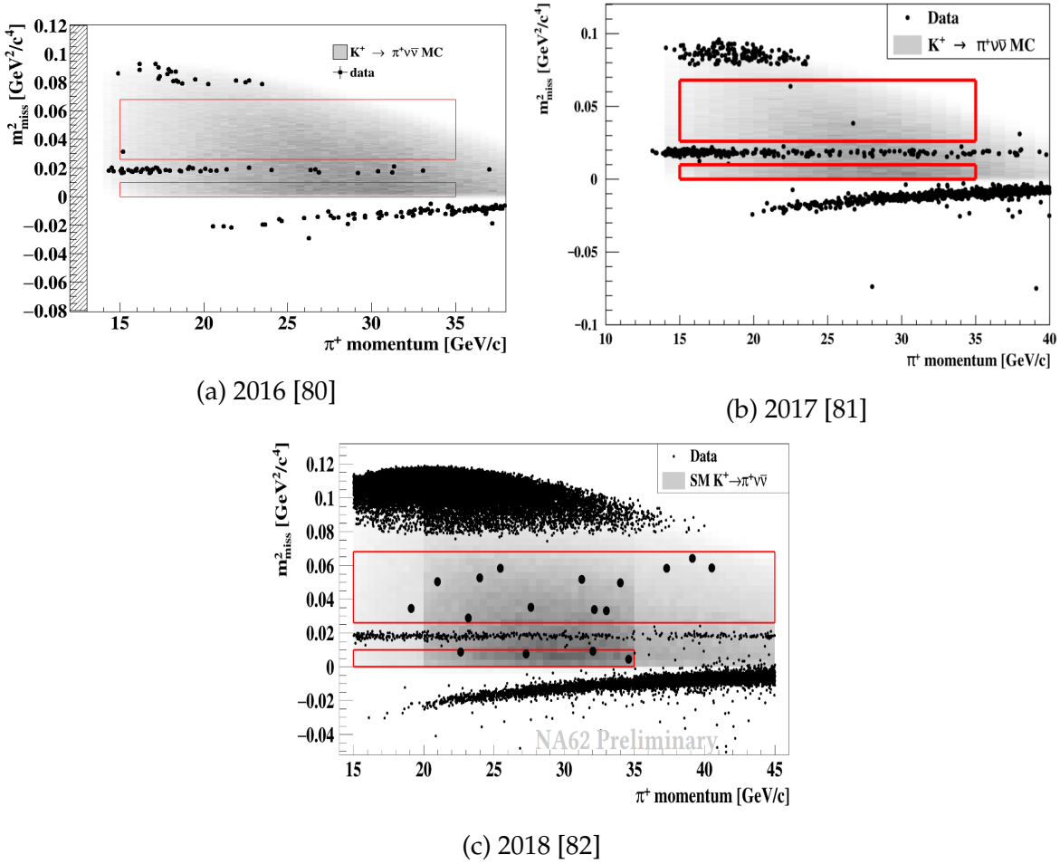
Figure 1.2.8: NA62 results of the K_{\pi\nu\nu} measurement from the first three years of data taking. Red rectangles correspond to the K_{\pi\nu\nu} signal regions. Signal event candidates in the 2018 plot are enlarged for better visibility.
