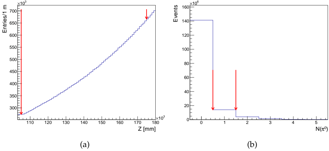
Figure 3.1.5: (a) Z position of the neutral vertex. (b) Number of \pi^0 candidates. Exactly one reconstructed \pi^0 candidate is required in K_{2\pi} and K_{\ell 3} selections. Data sample: 2017A, control trigger.
