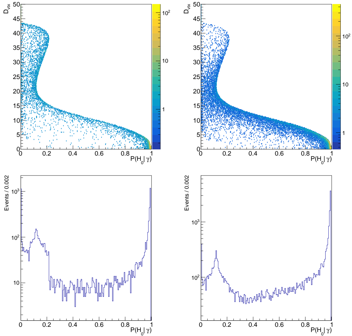
(a) K_{\mu 2}
